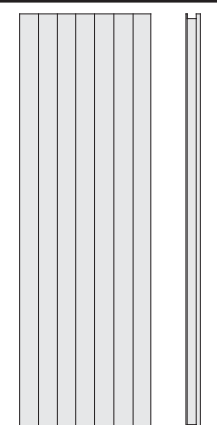
1 x W3 1920 x 606 x 57 mm ID 23624
